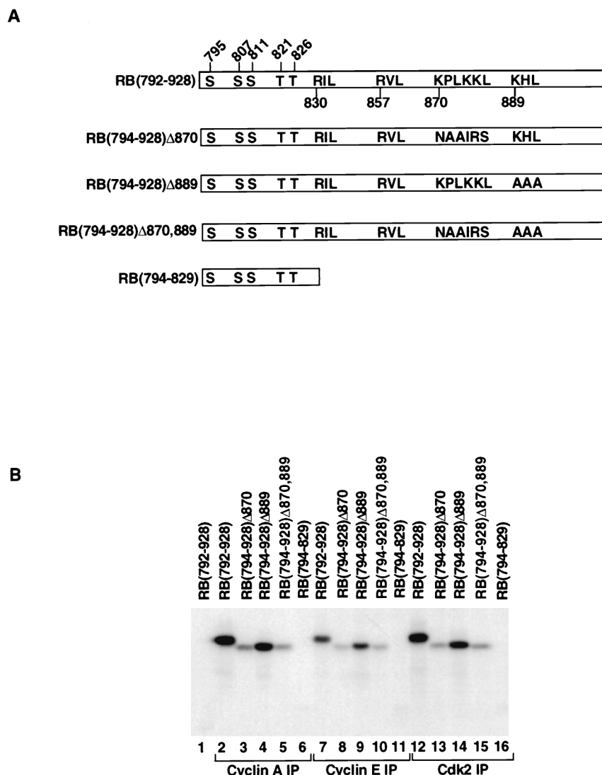
FIG. 3. A consensus cyclin-cdk binding motif between residues 870 and 875 mediates efficient phosphorylation of pRB. (A) Schematic illustrating the mutants used in the experiment in this figure. (B) U2OS osteosarcoma cells were lysed and immunoprecipitated with anti-cyclin A, anti-cyclin E, anti-cdk2, or control (lane 1, anti-SV40 T-antigen) antibodies as indicated. In vitro kinase assays were performed in the presence of 1 \mu g of the indicated GST-RB fusion proteins. Phosphorylated proteins were resolved by SDS-polyacrylamide gel electrophoresis, transferred to nitrocellulose, and detected by autoradiography. Comparable levels of the GST-RB proteins were confirmed by anti-GST Western blot analysis (data not shown).
